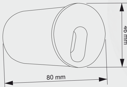
SL 8093 LED : 2x8W Color Temperature : 3000K,6000k Material: Die-casting Aluminum with Toughened Glass Body Color: Graphite Grey
