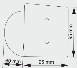
SL 8041 Square LED : 3W Color Temperature : 3000K,6000k Material: Die-casting Aluminum with ABS With Pc Diffuser Body Color: Graphite Grey
