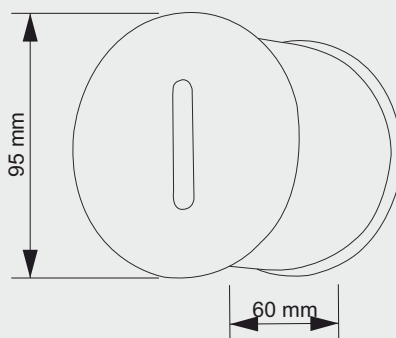
SL 8041 Round LED : 3W Color Temperature : 3000K,6000k Material: Die-casting Aluminum with ABS With Pc Diffuser Body Color: Graphite Grey
